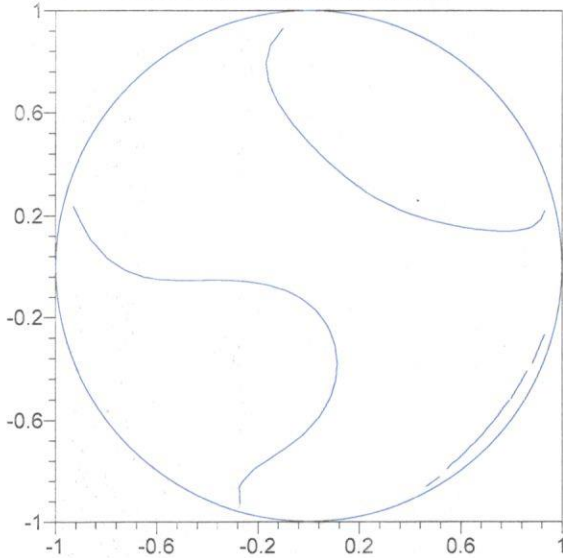
0.030 Micrometers / contour
